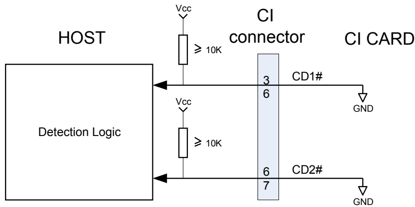
Figure K.1: Card Detect Mechanism
