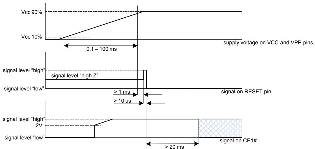
Figure K.2: Host supply power up timing diagram
