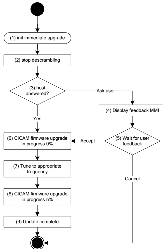
Figure 14.7: Immediate Process
