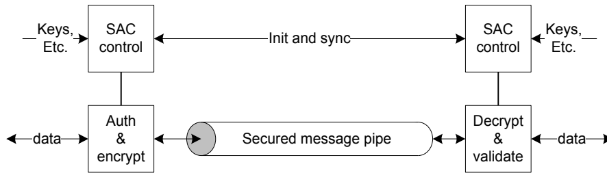
Figure 7.1: Contextual Overview of SAC (informative)
