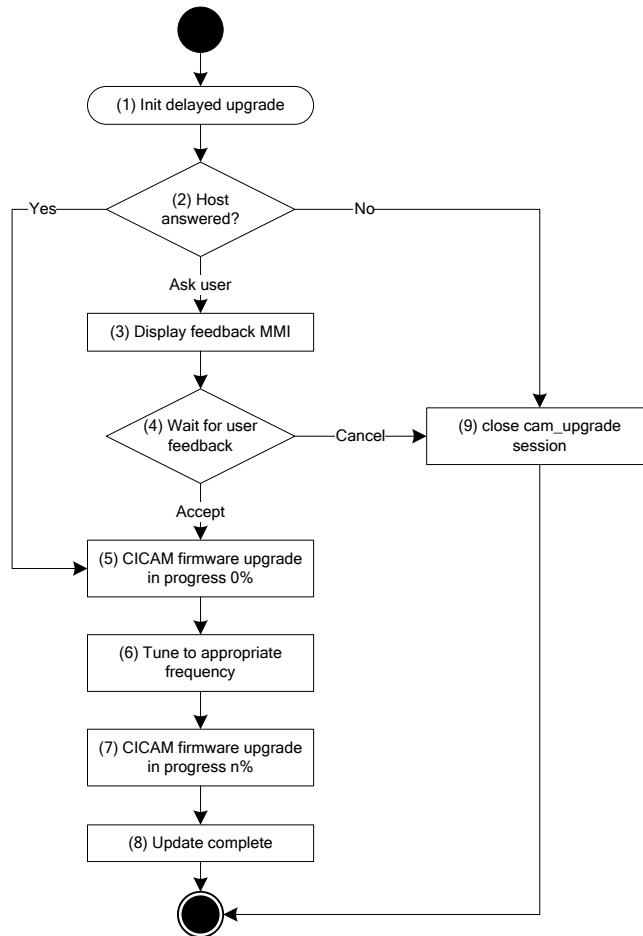
Figure 14.6: Delayed process
