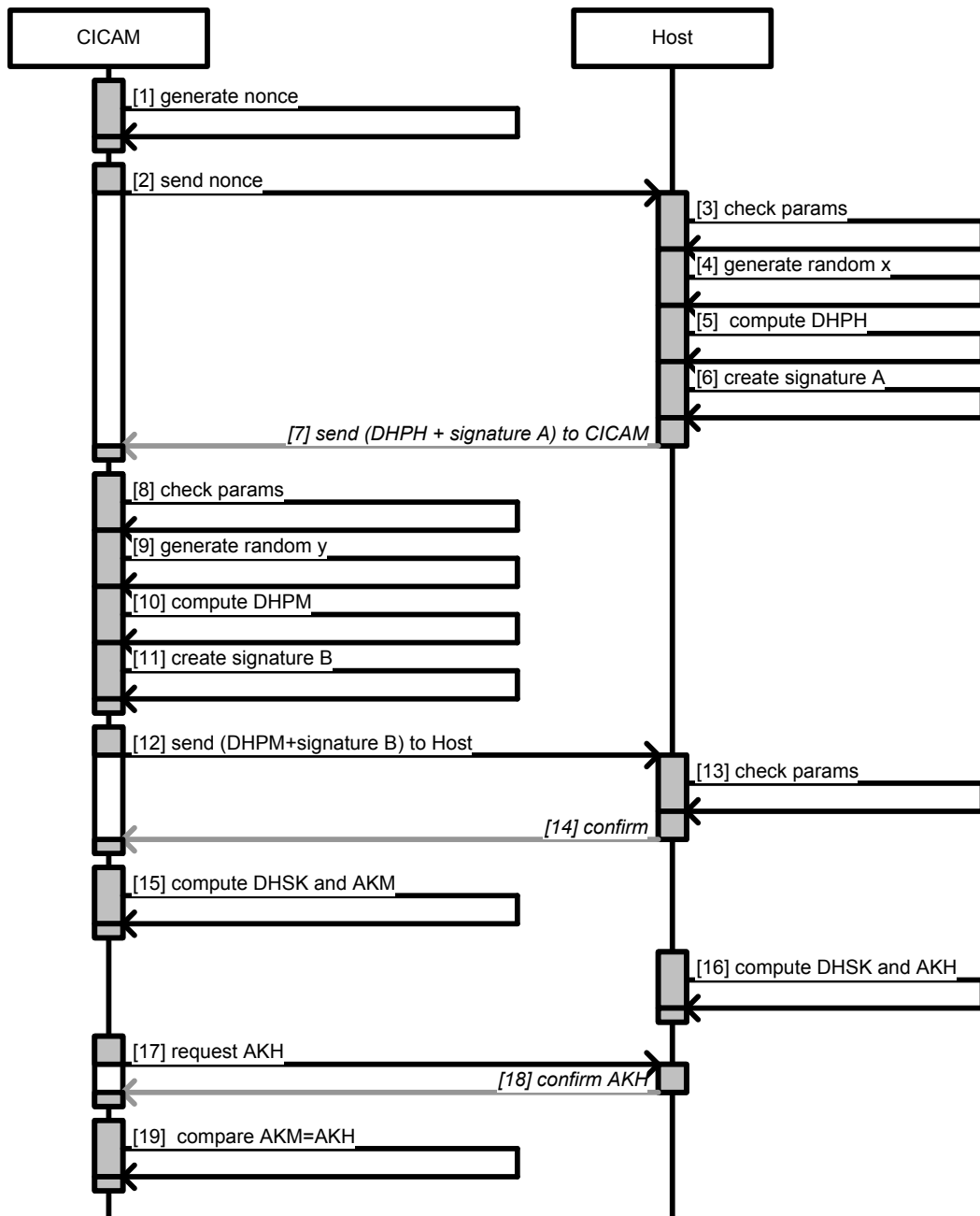
Figure 6.5: Authentication Key Material Computation Sequence Diagram (Informative)
