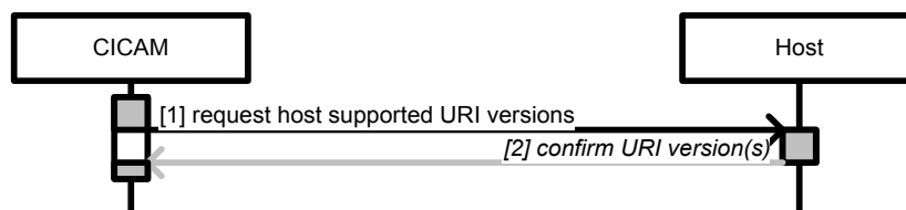
Figure 5.18: URI Version Negotiation Protocol
