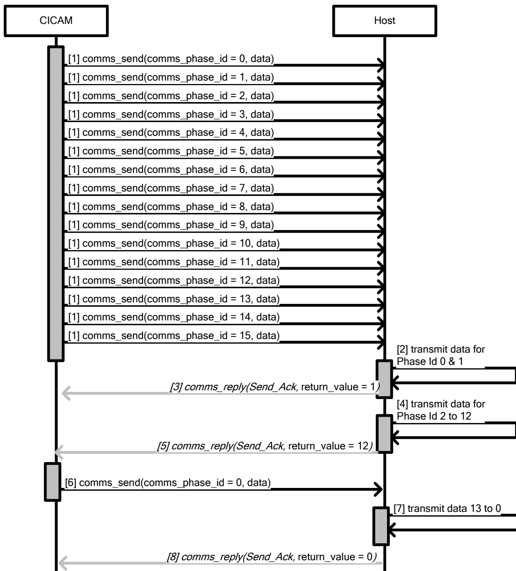
Figure 14.2: Host Flow Control with 16 buffers (Informative)
