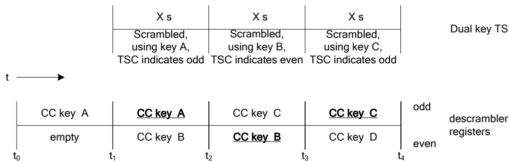
Figure 5.10: Relation between Descrambler Registers and TS
