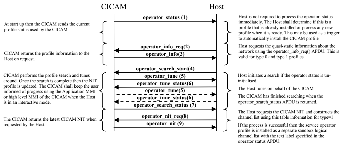
Figure 14.14: Profile Discovery APDU sequence
